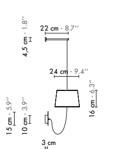
Tige murale / Fixed rod
